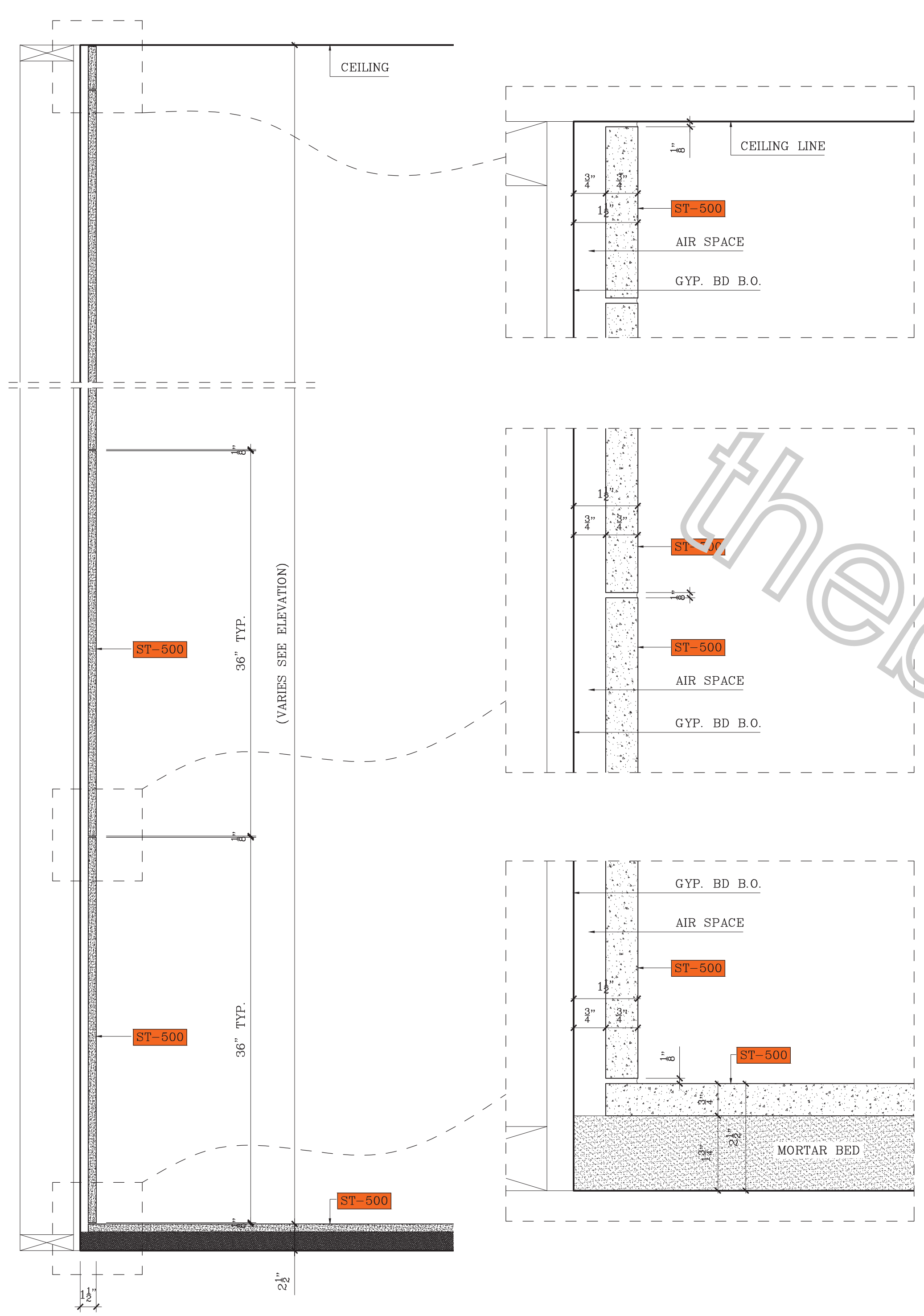
1 VERTICAL SECTION SCALE: 1 1/2"=1'-0"
