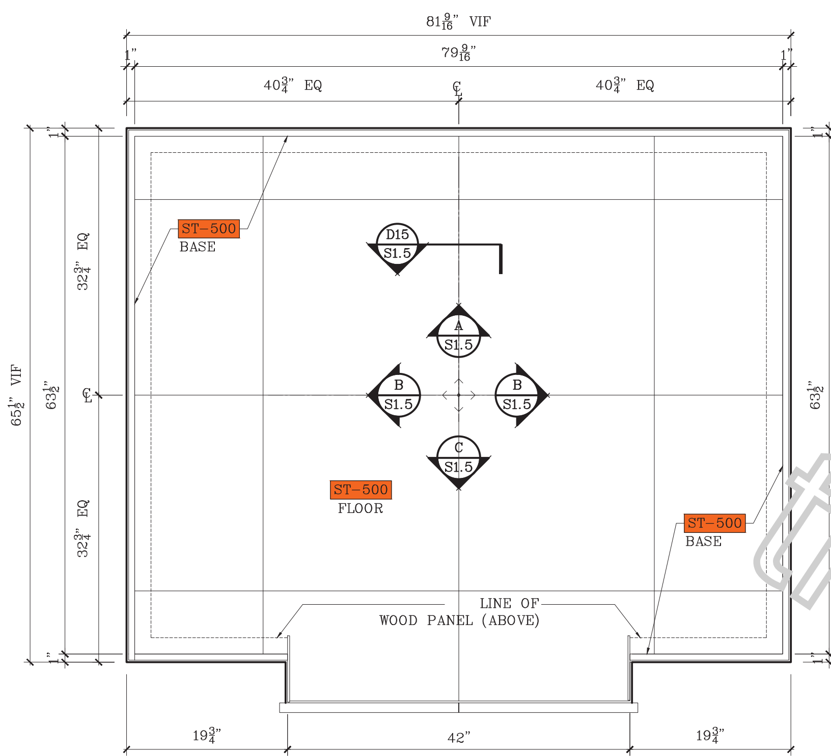
1 PLAN @ ELEVATOR CAB SCALE: 1"=1'-0"
